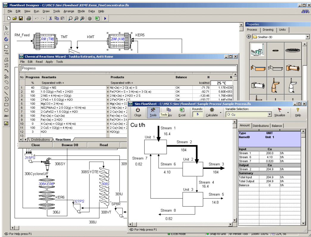
Fig. 2. HSC-Sim Module user interface.
